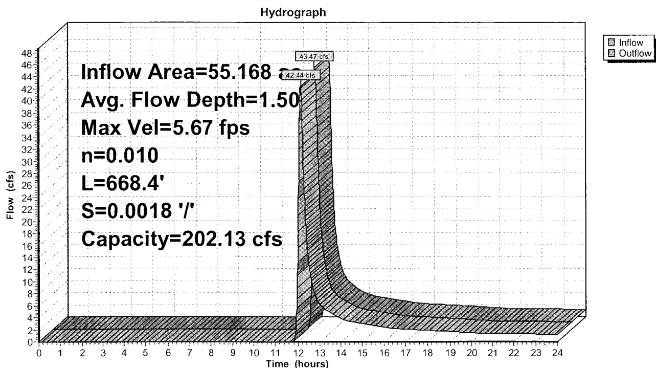
Reach 29R: Clean water diversion ditch
